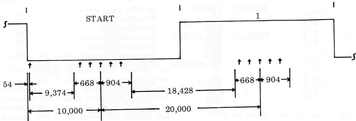
EXPANDED TIMING DIAGRAM
